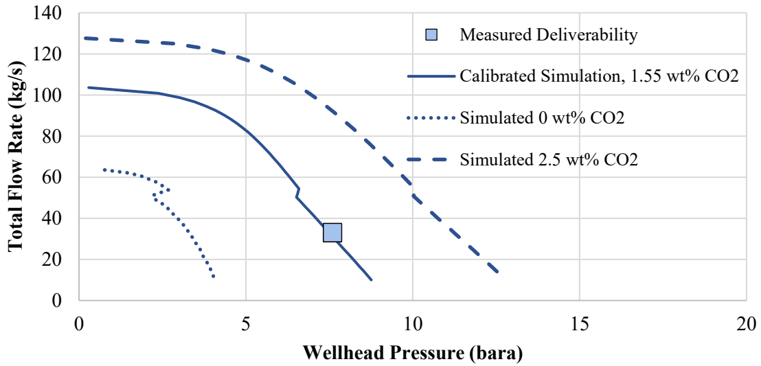
Figure 2: Calibrated Deliverability Curve and CO 2 Sensitivity
