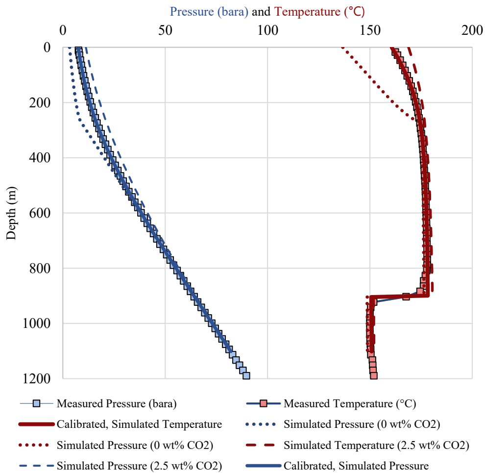
Figure 3: Measured and Simulated Temperature Flow Profiles for 1.55 wt% CO 2 Production Well and CO 2 Sensitivity. All profiles shown are at a flow rate of 33 kg/s per measurements.
