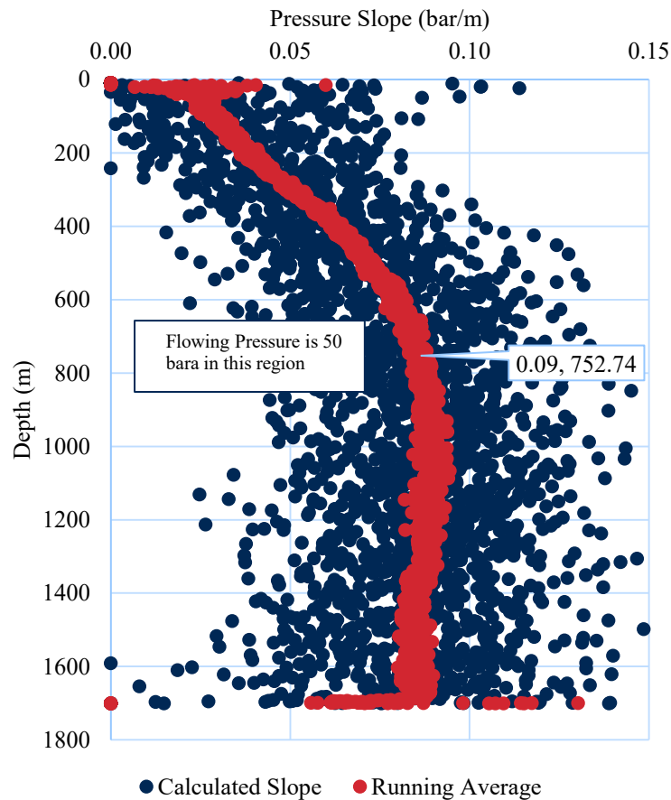
Figure 1: Pressure Change vs Depth for Example Flowing Well
