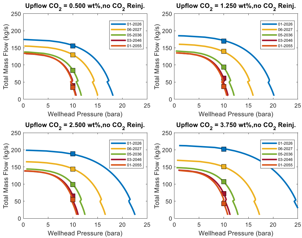
Figure 12: Deliverability Performance over Time, High Enthalpy Model
